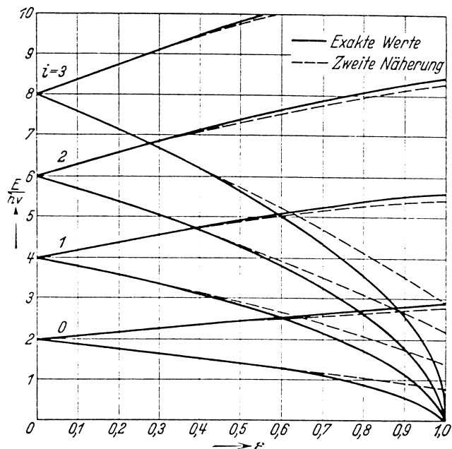
Fig. 1. Bending vibrational structure of the II-term for the total momentum M = 0 as a function of the interaction \epsilon .
