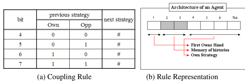
Fig. 2. An interaction rule of memory one
