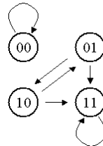
Fig. 4 The state transitions specified by the rule in Table 3.
