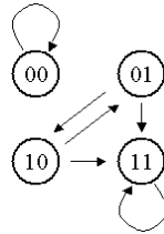
Fig. 6. The state transitions specified by rules in Table 6.
