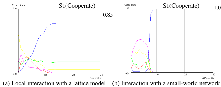
Fig. 3 The ratio of cooperation in iterated dilemma games
