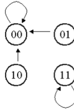
Fig. 8. The state transitions specified by rules in Table 8
