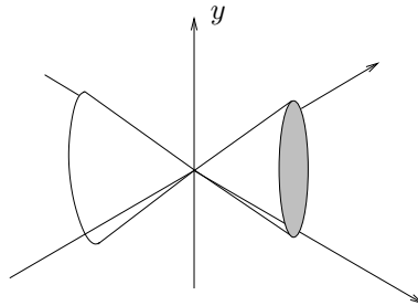
Figure 1. The set of real points of Y
