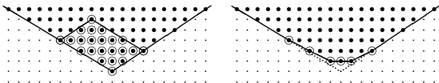
Figure 5. Fundamental cell P_\gamma and polyhedron K_\gamma for \gamma = \text{cone}(-5e_1 + 3e_2, 3e_1 + 2e_2)
