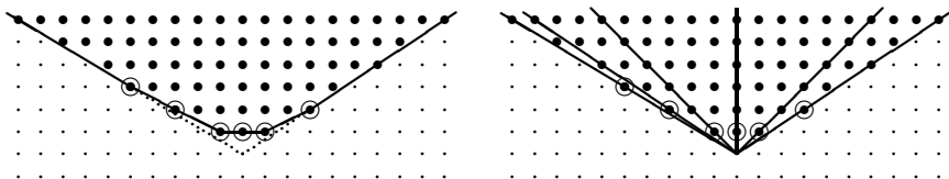
Figure 16. Polyhedron K_\sigma and minimal resolution for \sigma = \text{cone}(-5f_1 + 3f_2, 3f_1 + 2f_2)
