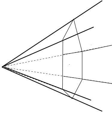
Figure 4. A strongly convex polyhedral cone and its faces
