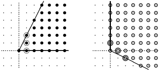
Figure 8. A pair of dual cones \gamma, \gamma^\vee for dual lattices L, L^*
