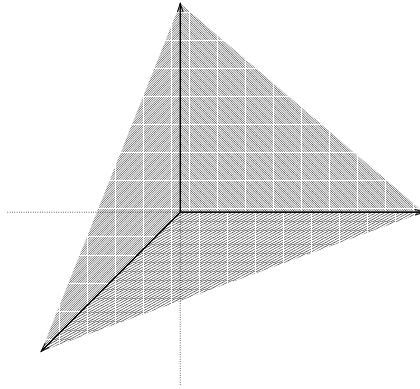
Figure 12. The fan for the projective plane \mathbb{P}_2
