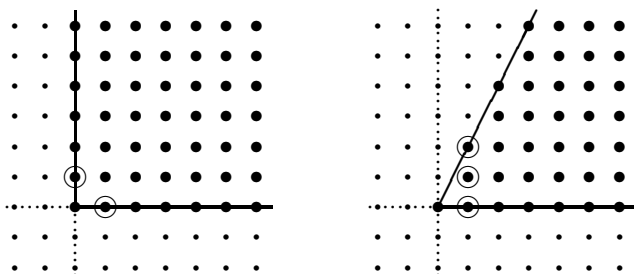
Figure 6. The M -cones cutting out E_{\mathbb{C}^2} and E_Y (cf. Figure 3)
