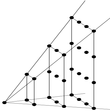
Figure 7. The M -cone \gamma = \text{cone}(e_1, e_2, e_1 + e_3, e_2 + e_3) cutting out E_Z
