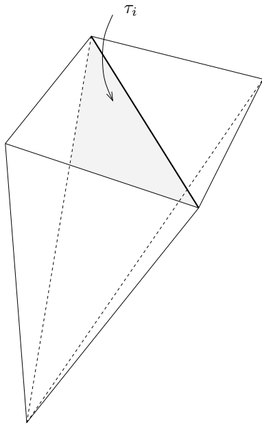
Figure 19. A thin simplicial subdivision
