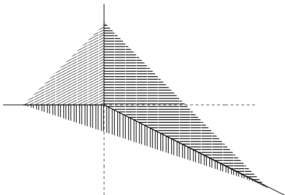
Figure 14. The fan for the projective quadric cone
