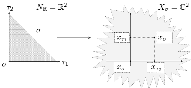
Figure 10. Faces of \text{cone}(f_1, f_2) and corresponding orbit base points in \mathbb{C}^2
