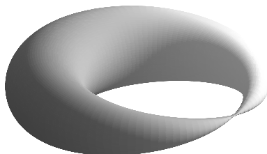
Figure 15. The set of real points of the projective quadric cone
