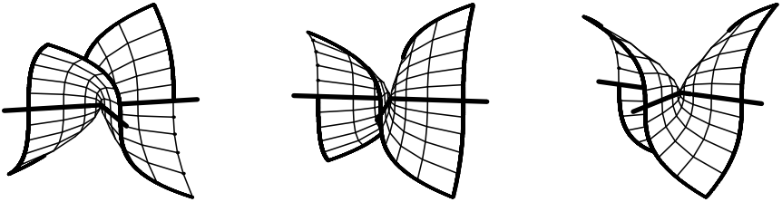
Figure 2. Three views of the set (Y_3)_{\mathbb{R}} with the real A_2 surface singularity
