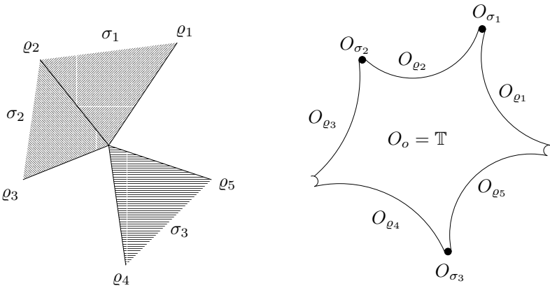
Figure 13. Correspondence between fan cones and orbits
