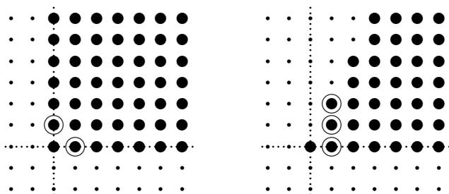
Figure 3. Points and generators of E_{\mathbb{C}^2} and of E_Y
