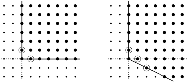
Figure 9. The N -cones for \mathbb{C}^2 and Y
