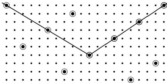
Figure 11. Sublattice \Gamma_\sigma for \sigma = \text{cone}(-5f_1+3f_2, 3f_1+2f_2)
