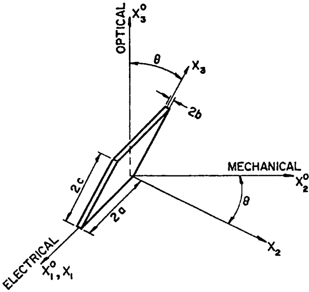
Fig. 1.041 Rotated x_2 -cut of quartz.
