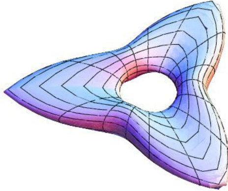
Figure 8. Hyperbolic orbifolds.
