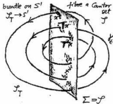
Figure 12. Mapping torus.
