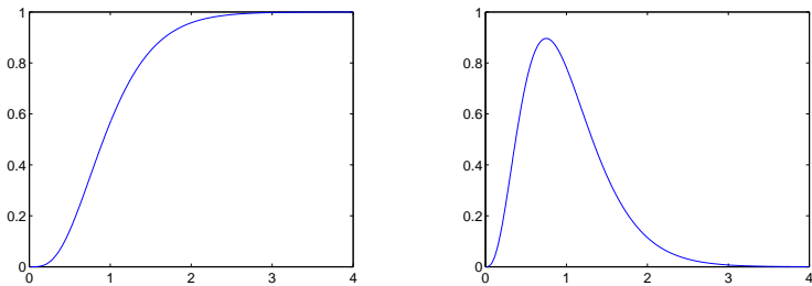
Fig. 1.2 The continuous \text{Gamma}(4, 0.25) distribution function (left) and its density (right).
