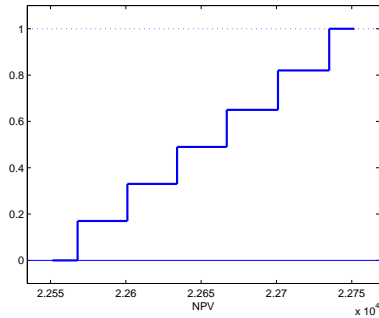
Fig. 1.1 The discrete distribution function of the data in Table 1.2.
