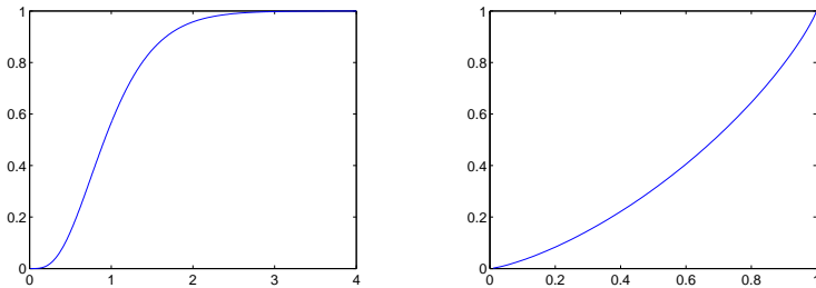
Fig. 1.8 Left: the distribution function \text{Gamma}(4, 0.25, 0) Right: the pertaining Lorenz curve
