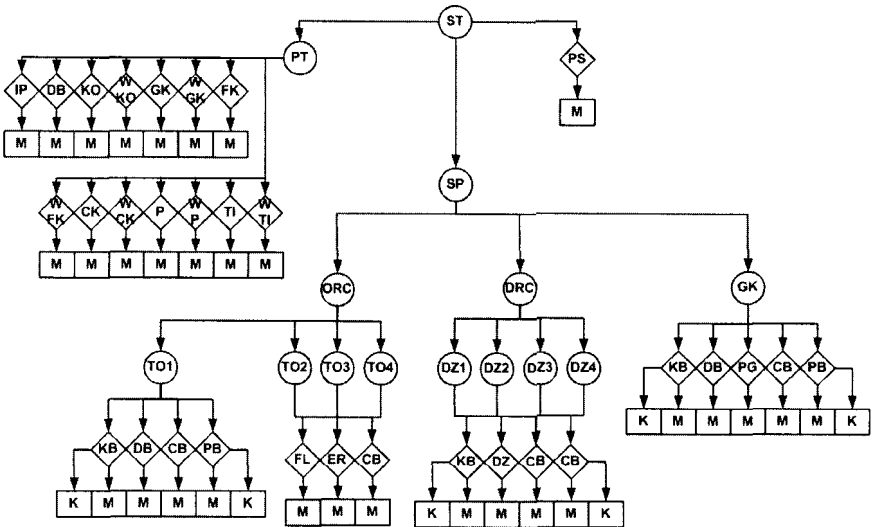
Figure 4. Overall view of a HDM developed for soccer-playing robots.
