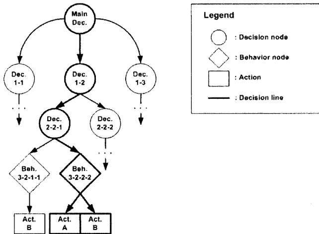
Figure 2. Graphical representation of the Hierarchical Decision Machine.
