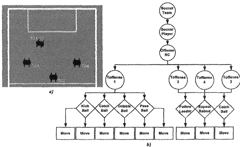
Figure 5. Dynamic offensive formation (a) and corresponding decision machine (b).
