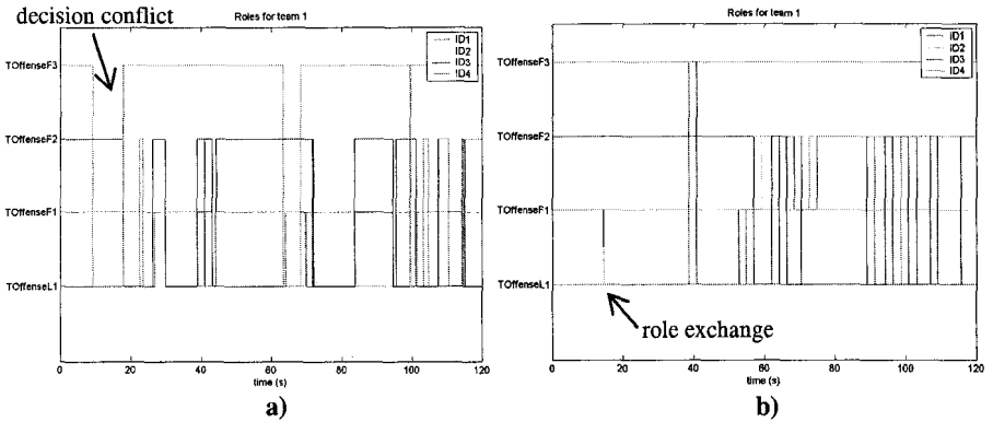
Figure 6. Dynamic role allocation without (a) and with (b) supervision.
