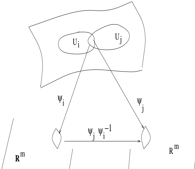
Fig. 1.2 Transition maps
