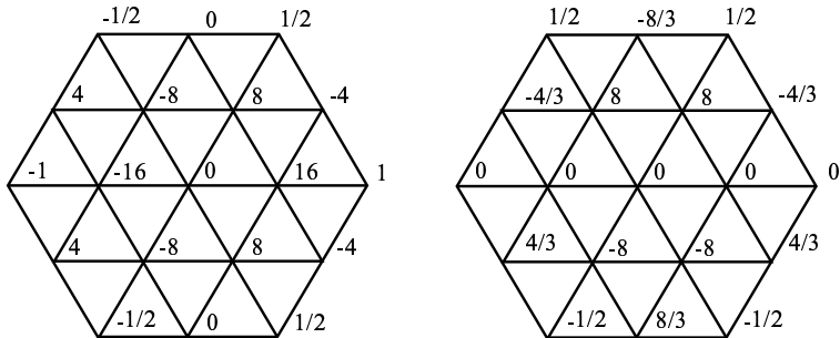
Fig. 8. Tangent masks for regular vertices (Butterfly scheme).
