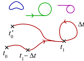
Fig. 3. Configuration space showing the limit cycles of an evolving system, indicating the times t_0, t_1 and the period \Delta t of a limit cycle. The points at t_0 and t'_0 form one equivalence class.
