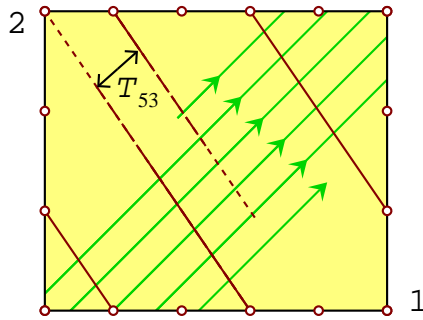
Fig. 2. The equivalence class for oscillators in the case (p, q) = (5, 3) . Lines with arrows pointing right and up: time trajectories of individual points. Solid and broken lines going downwards: (part of) the (5, 3) equivalence class at t = 0 . For further explanation, see text.
