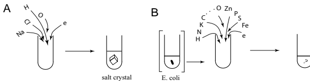
Fig. 1.1 Analogue experiments to distinguish simple and complex systems.
