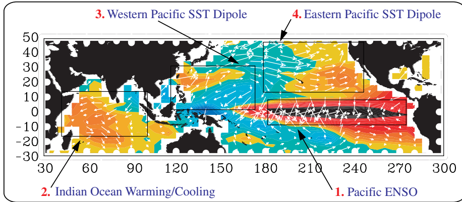
Figure 4. Structures of SST and surface wind stress anomalies of the leading M-SSA mode obtained from the Indo-Pacific Run. Contours represent SST anomalies. Surface wind stress anomalies are indicated by vectors. Contour intervals are 0.1^{\circ}\text{C} . The structures shown are taken from the mature phase of ENSO in the leading M-SSA mode.
