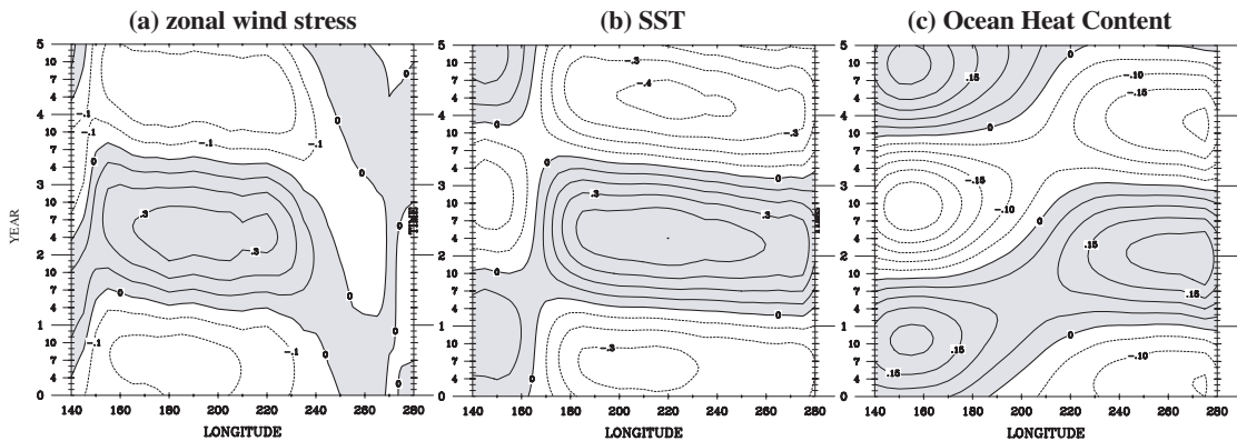
Figure 2. Structures of the simulated ENSO cycle along the equatorial Pacific extracted from the Pacific Run by the M-SSA method. Panel (a) shows the structure of zonal wind stress anomalies, (b) the structure of SST anomalies, and (c) the structure of ocean heat content anomalies. The coordinate is the 61-month (5-year) lag used in the M-SSA. Contour intervals are 0.1 \text{ dyn/cm}^2 for (a), 0.10^{\circ}\text{C} for (b), and 0.05^{\circ}\text{C} for (c). Values shown in (a) are scaled by 10. Positive values are shaded. (From Yu and Mechoso, 2001.)
