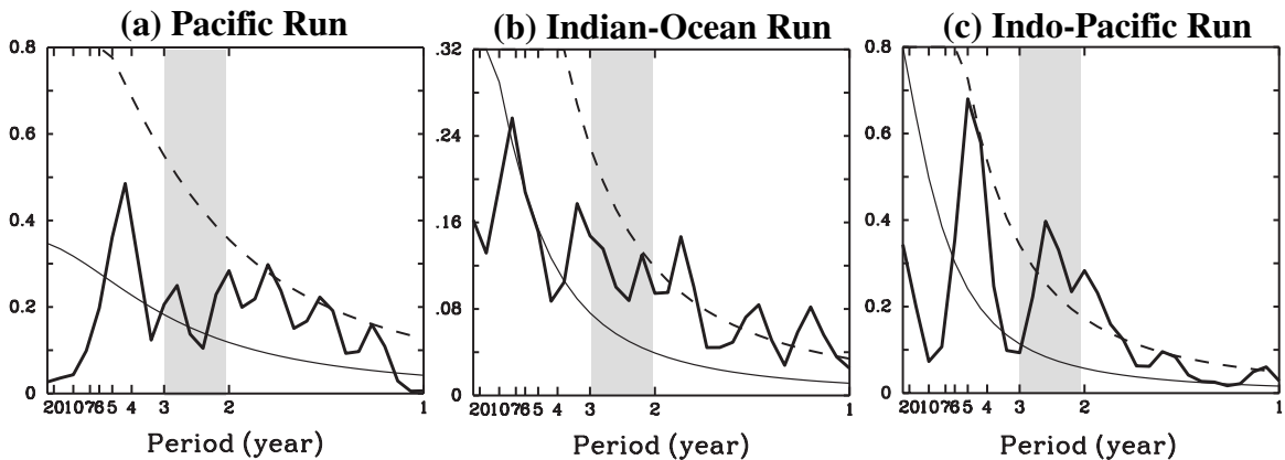
Figure 9. Power spectra of the Indian summer monsoon rainfall index calculated from the (a) Pacific Run, (b) Indian-Ocean Run, and (c) Indo-Pacific Run. The 95% significance levels are indicated by the dashed curves. The shaded area is the period for the quasi-biennial oscillation.
