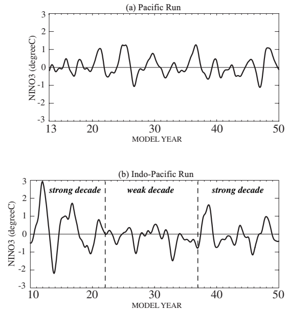
Figure 6. NINO3 SST anomalies calculated from (a) the Pacific Run and (b) the Indo-Pacific Run. These monthly values are low-pass filtered to remove variations shorter than 12 months. (From Yu et al. , 2002.)
