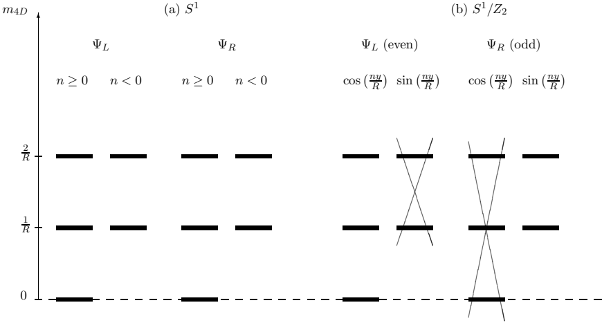
Fig. 1.3. KK decomposition for a 5D fermion on a circle (a) and an orbifold (b) with even parity for \Psi_L .
