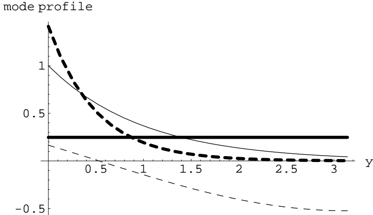
Fig. 1.8. Same as Fig. 1.7, but with brane kinetic term, r/R = 10 , for gauge fields on y = 0 brane.
