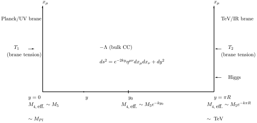
Fig. 1.12. The Randall-Sundrum (RS1) model.
