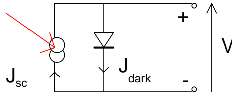
Fig. 1.7. Equivalent circuit of ideal solar cell.
