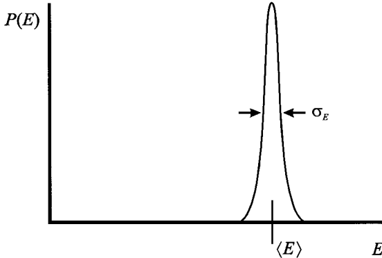
Fig. 1.7. Fluctuations in energy for a system at fixed temperature.
