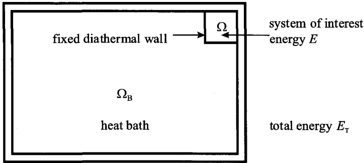
Fig. 1.4. Thermal interaction with the rest of the world.
