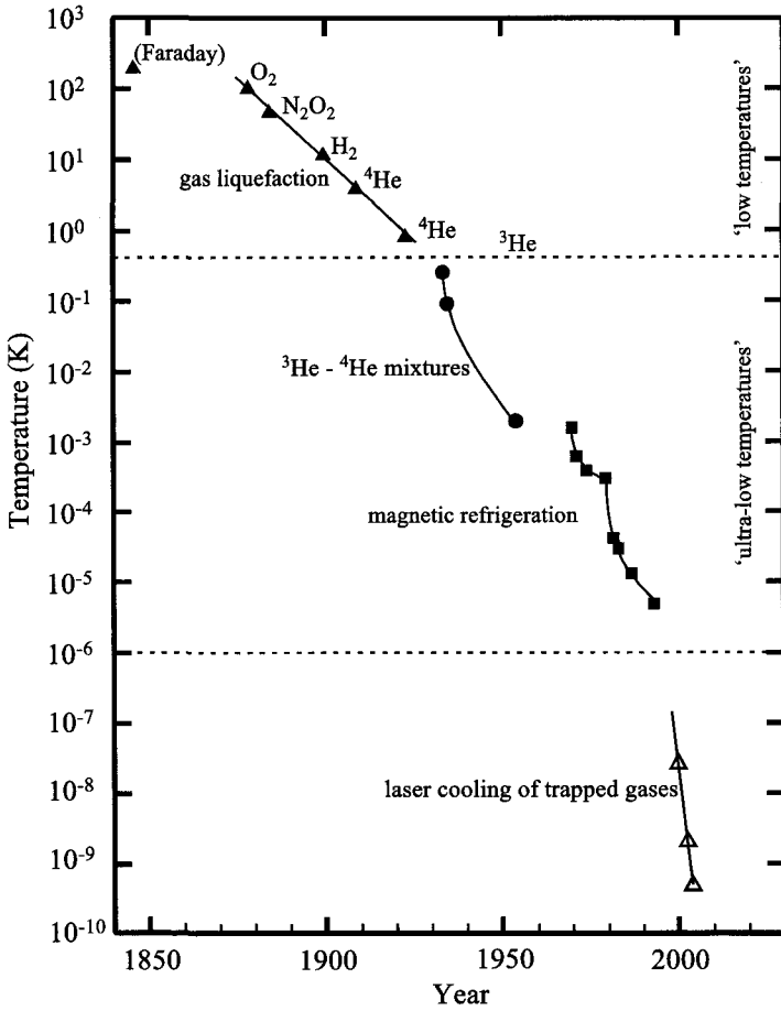
Fig. 1.14. The road to absolute zero.
