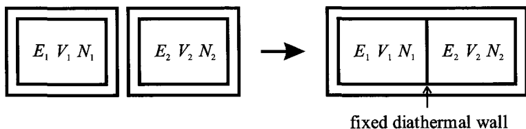
Fig. 1.1. Thermal interaction.
