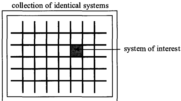
Fig. 1.6. Gibbs* ensemble for evaluating generalised entropy.
