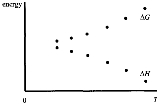
Fig. 1.12. Nernst's observations.
