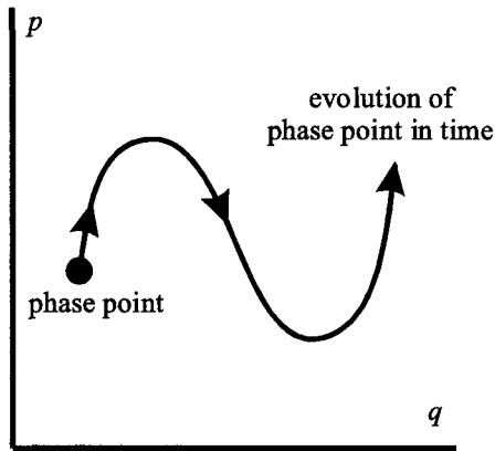
Fig. 1.9. Phase space.
