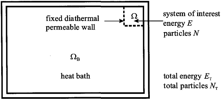
Fig. 1.5. Particle and energy exchange with the rest of the world.
