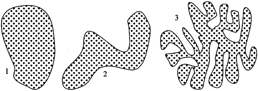
Fig. 1.10. Evolution of a region of phase space.
