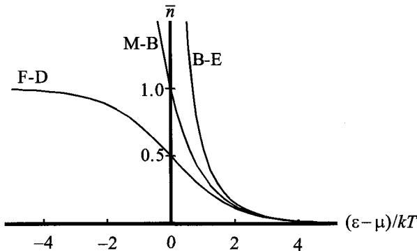
Fig. 1.8. Fermi–Dirac, Maxwell–Boltzmann and Bose–Einstein distribution functions.
