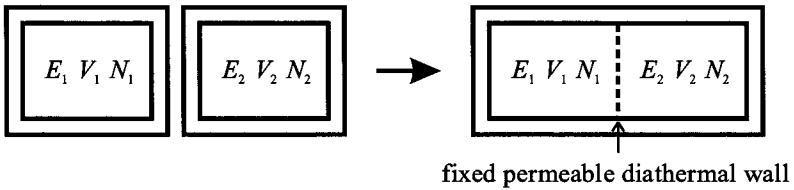
Fig. 1.3. Heat and particle exchange.
