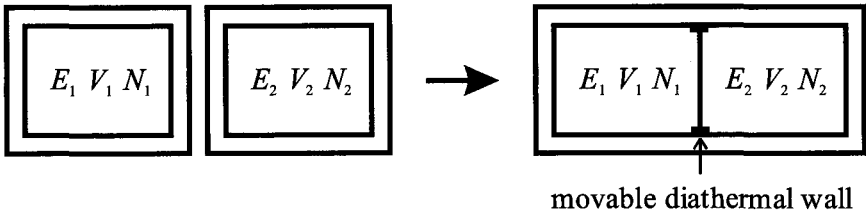
Fig. 1.2. Mechanical and thermal interaction.
