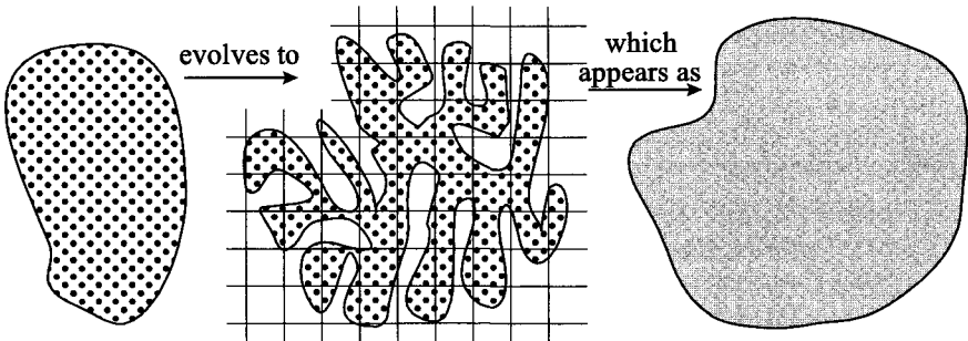
Fig. 1.11. Apparent reduction in density in phase space.
