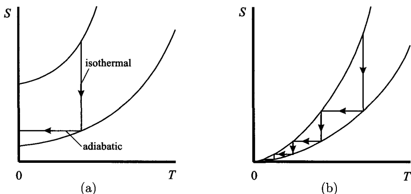
Fig. 1.13. Approaching absolute zero. System (a) not obeying the Third Law can get to T = 0 in two steps. System (b) obeying the Third Law cannot get to T = 0 in a finite number of steps.
