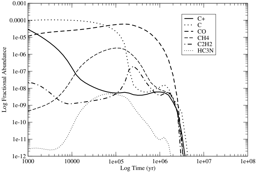
Fig. 1.2. Time evolution of gas-phase carbon chemistry but with accretion at T = 10 K and n = 10^4 \text{ cm}^{-3} .
