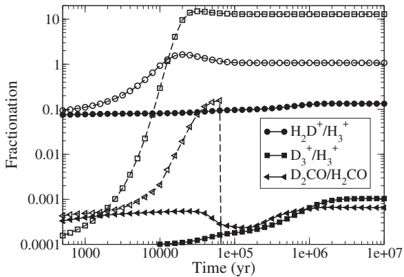
Fig. 1.3. Fractionation ratios plotted against time for a cloud with \text{H}_2 density 10^6 \text{ cm}^{-3} and temperature 10 K. Results with unfilled objects are for the case of grain accretion, whereas those with filled objects are for the case of no grain accretion. Calculation performed by Dr. Helen Roberts.
