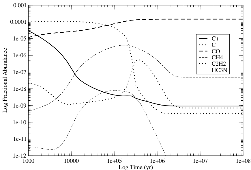
Fig. 1.1. Time evolution of gas-phase carbon chemistry at T = 10 K and n = 10^4 cm ^{-3} .
